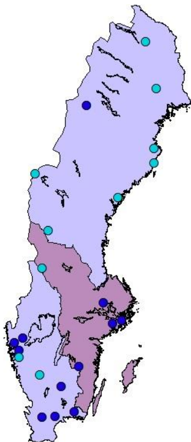
(a) \text{NO}_3^- + \text{NH}_4^+ deposition TRENDMATCH
